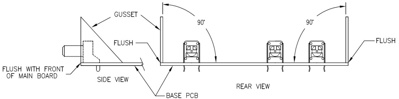
Both sides 90°, ready for next step
